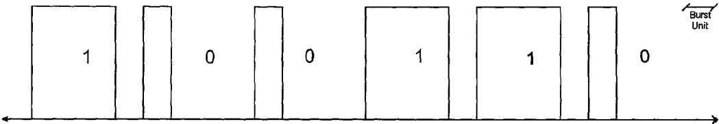
FIGURE 2b - Fixed Bit Time, Burst Width Modulated
