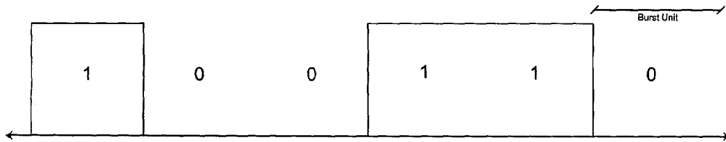
FIGURE 2a - Fixed Bit Time, Full Width Burst
