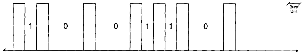
FIGURE 2f - Fixed Burst Time, Off Time Modulated
