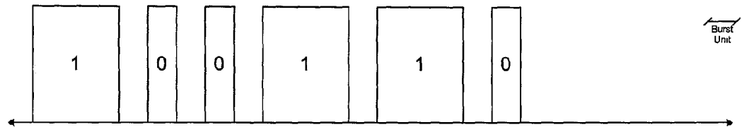
FIGURE 2c - Fixed Off Time, Burst Width Modulated
